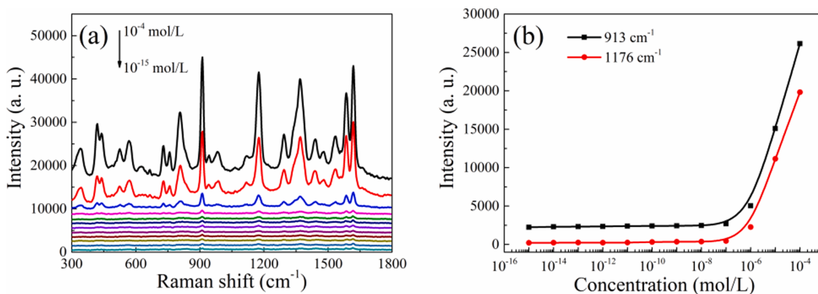
Fig. 4. (a) SERS spectra of crystal violet with different concentrations adsorbed on silver nanowires arrays. (b) The relationship between crystal violet concentrations and peak intensities at 913 and 1176 cm -1 .
