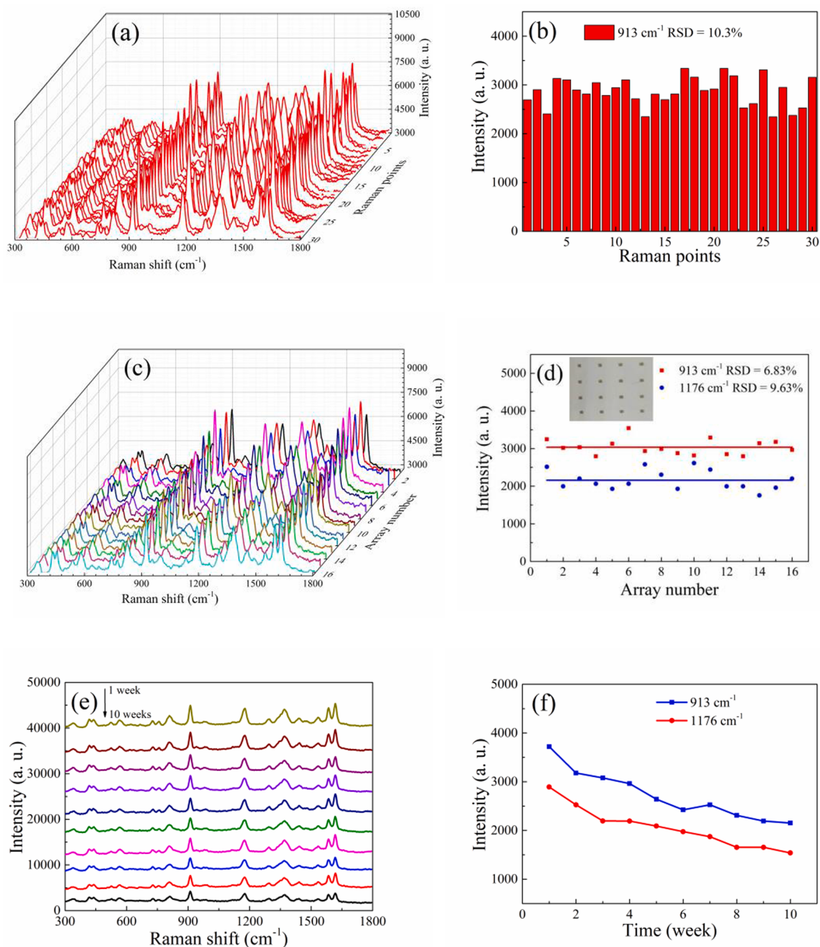
Fig. 5. (a) SERS spectra of thirty points of crystal violet adsorbed on the same array and (b) the corresponding SERS intensity distribution at 913 cm -1 . (c) SERS spectra of crystal violet obtained from 4 × 4 silver nanowire arrays and (d) the corresponding SERS intensities at 913 and 1176 cm -1 . (e) SERS spectra of crystal violet during different storage time and (f) the corresponding SERS intensities at 913 and 1176 cm -1 .
